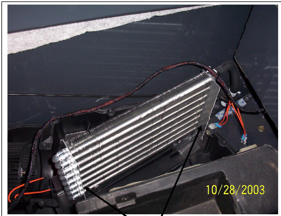
Cut existing aluminum flanges down to about 1" using metal snips
